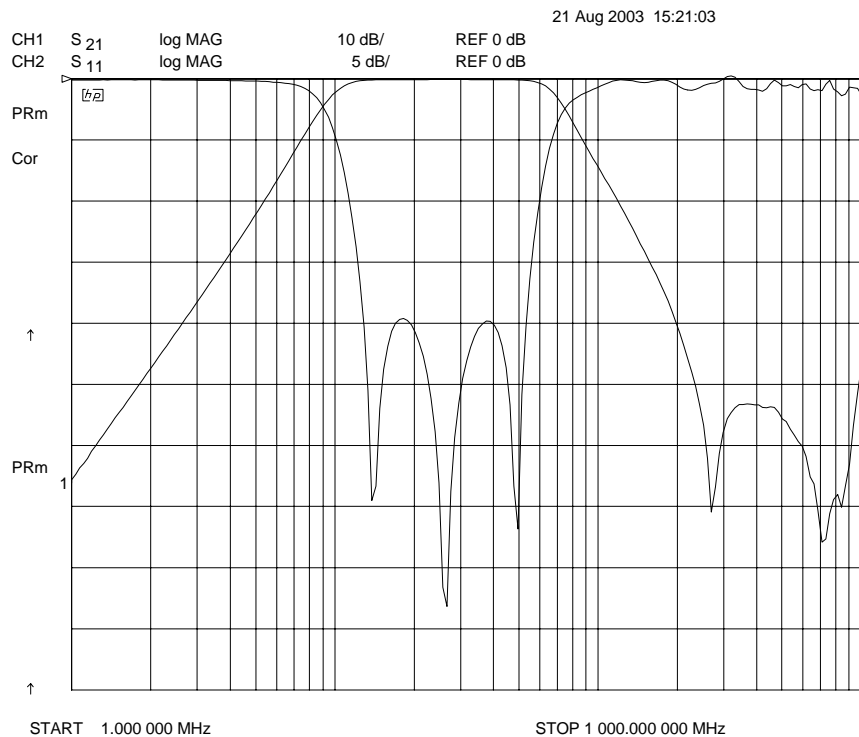
Overall Response & Return Loss (10 dB/div & 5 dB/div)
